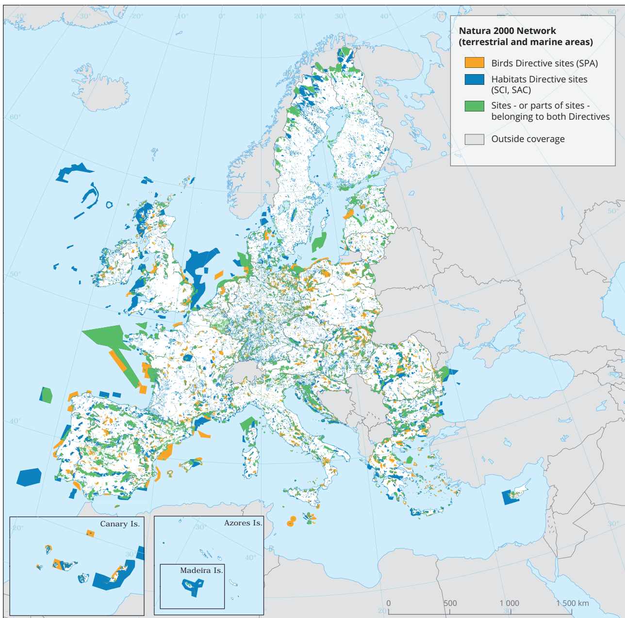
Map 5.3 Natura 2000 network (terrestrial and marine areas)
